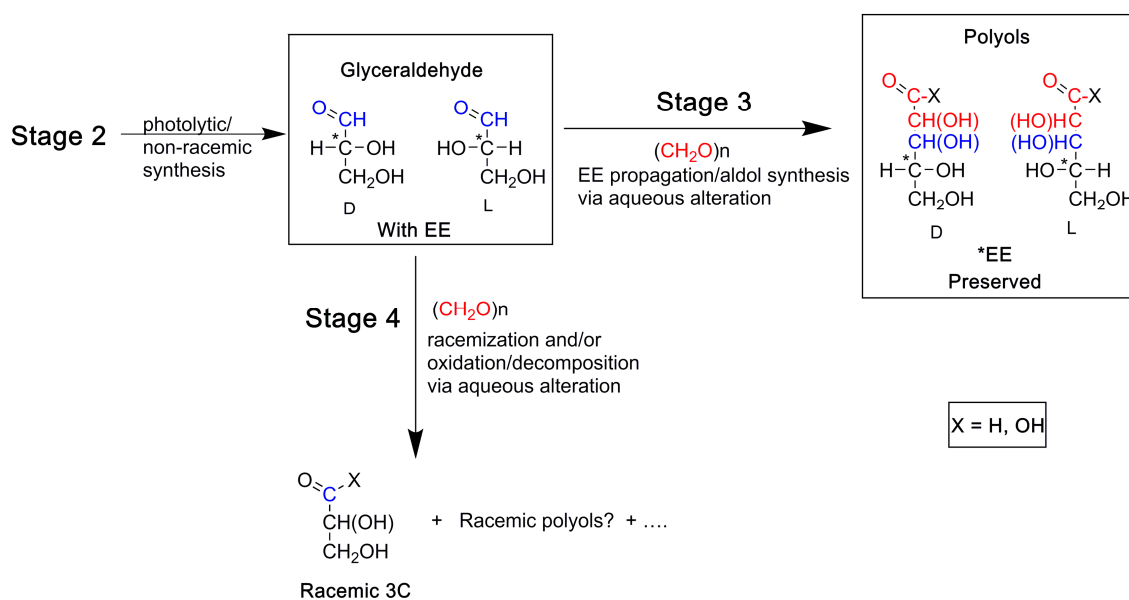
Scheme 3. Possible fate of a non-racemic fraction of glyceraldehyde during aqueous alteration. Glyceraldehyde is pictured as reacting with formaldehyde ( n = 1 ) or glycolaldehyde ( n = 2 ) to produce larger polyols with enantiomeric excess ( ee ). If X = \text{H} , 5C sugars are the products; If X = \text{OH} , 5C sugar acids are the (oxidation) products. However, glycolaldehyde by itself readily produces sugars (especially 4C sugars), and likely even under the weak formose conditions of meteorite parent bodies (Section 3.1).
