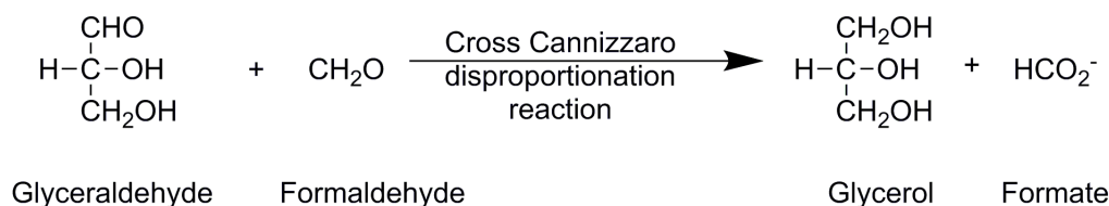
Scheme 1. The production of glycerol in the crossed-Cannizzaro reaction [14].
