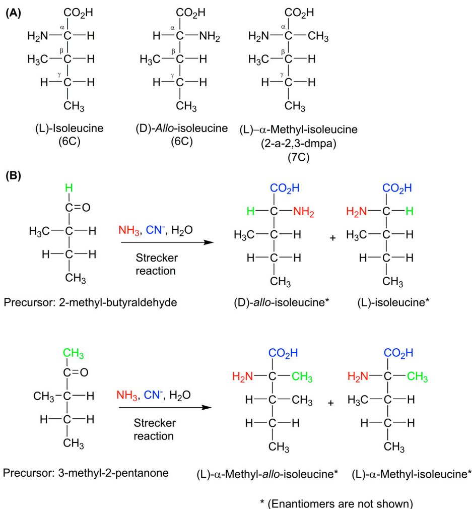
Scheme 2. (A) The structural relationship between isoleucine, allo -isoleucine and \alpha -methyl-isoleucine; (B) An illustration of obtaining specific diastereomers in the same Strecker reaction. Each diastereomer has its own enantiomer ratio. From the structures of allo -isoleucine and isoleucine it can be seen that they are not mirror images (enantiomers) of each other. Instead, they are epimers, i.e., stereoisomers that have multiple chiral centers, but only differ from one another by the configuration at one of the chiral centers. It is much easier to epimerize either compound into the other by inverting the stereochemistry at the \alpha carbon because it contains an exchangeable hydrogen. However it is much more difficult to invert both \alpha and \beta carbons of a given compound to obtain its enantiomer (see text).
