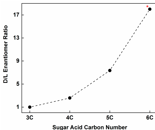
Figure 4. The D/L enantiomeric ratios of meteoritic aldonic acids (Figure 3) increase with carbon number [31]. The asterisk shown in the 6C value is extrapolated based on the D/L trend of 3C \rightarrow 4C sugar acids as reported in [31].
