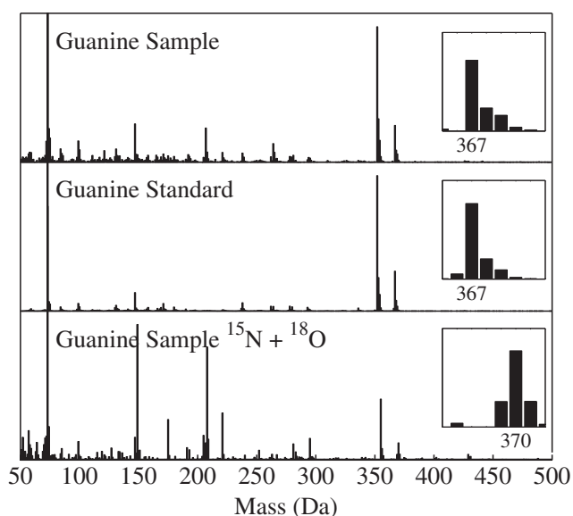
FIG. 4. Top panel: (Top trace) TIC of the residue produced from a UV-irradiated \text{H}_2\text{O}:\text{NH}_3 :purine ice. (Middle trace) SIC of the same residue for mass 367 Da. (Bottom trace) SIC of the guanine standard (mass 367 Da). Bottom panel: (Top trace) Mass spectrum of the peak identified as guanine in the residue produced from a UV-irradiated \text{H}_2\text{O}:\text{NH}_3 :purine ice. (Middle trace) Mass spectrum of a guanine standard. (Bottom trace) Mass spectrum of the peak identified as guanine in the residue produced from a UV-irradiated ice containing \text{H}_2^{18}\text{O} and ^{15}\text{NH}_3 instead of \text{H}_2\text{O} and \text{NH}_3 , respectively. The observed mass increase matches what is expected for the guanine identification.
