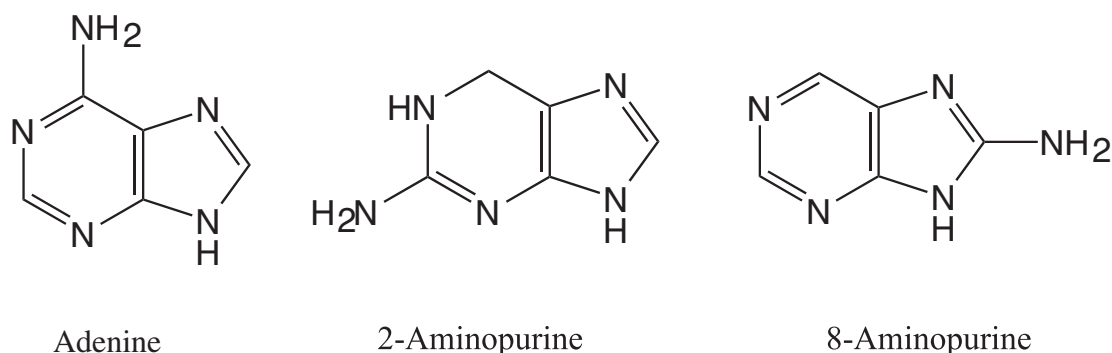
FIG. 5. Structures of all possible singly aminated purines. The presence of adenine and 2-aminopurine have been confirmed using GC-MS by comparison with a commercial standard. 8-Aminopurine is hypothesized to also be present based on the mass spectra of several unidentified peaks in the chromatogram. However, no standards were commercially available for confirmation.
