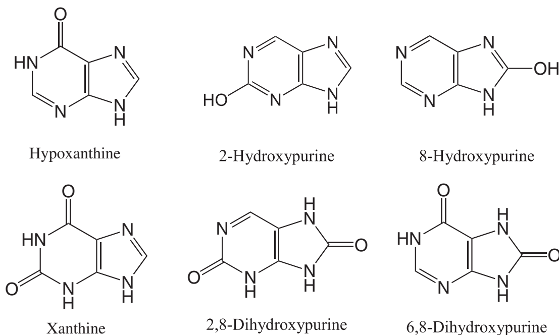
FIG. 2. Structures of all possible singly and doubly oxidized purines ( N -oxides excluded). The presence of hypoxanthine and xanthine have been confirmed using GC-MS by comparison with commercial standards. The remaining four compounds are hypothesized to also be present based on the mass spectra of several unidentified peaks in the chromatogram. However, no standards were commercially available for confirmation.
