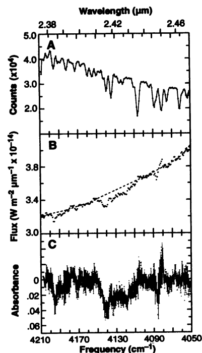
Fig. 1. The spectrum from 4210 to 4050 \text{cm}^{-1} ( 2.38 to 2.47 \text{ }\mu\text{m} ) of (A) the unratified spectrum of the comparison star BS 5953, (B) the spectrum of WL5 after ratioing by BS 5953, and (C) the optical depth plot of WL5 derived with the continuum base line (dashed trace) shown in (B). The spectrum in (C) has been smoothed using a Gaussian with a FWHM of 1.5 data points (1/2 resolution element) and results in a resolution of \sim 3 \text{ cm}^{-1} (19).
