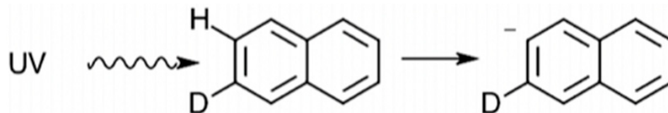
Scheme 1. Unimolecular photodissociation.
