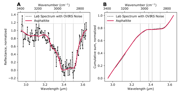
Fig. A.4. Example of the two fitting methods developed in two previous studies (Kaplan et al. 2020; Ferrone et al. 2021): (a) linear least-squares fitting of normalized data and (b) a Kolmogorov-Smirnov fitting method, in which we search for the maximum distance between the two curves. The black curves are laboratory data with noise added to simulate OVIRS noise, and the red curves are laboratory data at their original S/N. Vertical lines at 3.10 , 3.275 , 3.38 , 3.42 , and 3.50\ \mu\text{m} indicate positions of possible absorption features.
