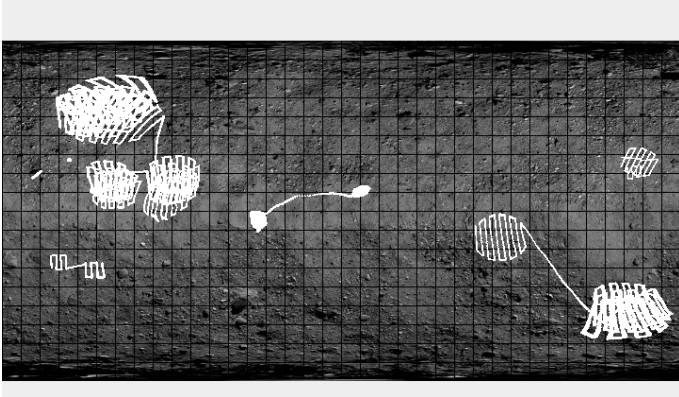
Fig. A.1. OVIRS footprints from the Recon A phase of the OSIRIS-REx mission overlaid on a Bennu base map, which extends from -90^\circ to 90^\circ N and 0^\circ to 360^\circ E. There are 15 858 footprints shown on this map, which were analyzed for organic spectral features in this study.
