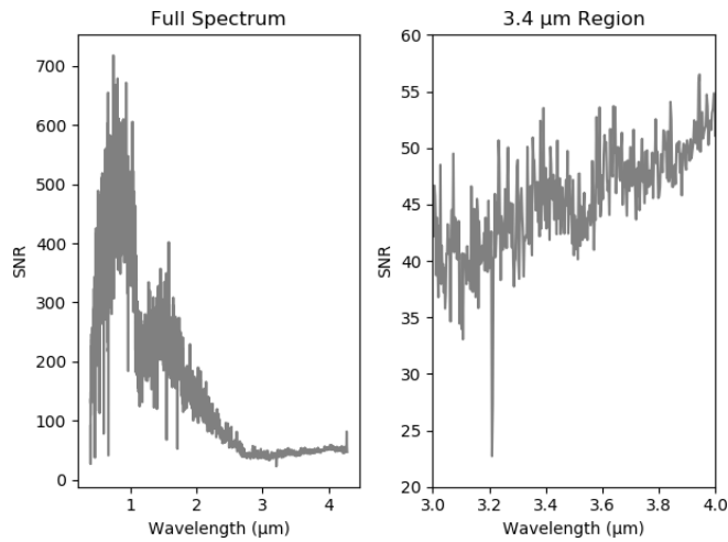
Fig. A.2. OVIRS S/N near 3.4\ \mu\text{m} , average for Recon A.
