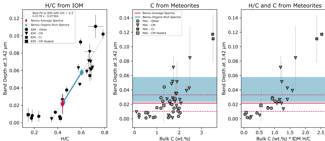
Fig. 3. Estimated H/C. (a) Carbonaceous chondrite IOM band depth at 3.42\ \mu\text{m} , plotted against H/C (atom.) from Alexander et al. (2007); “other” refers to IOM from CV, CO, CR, and ungrouped carbonaceous chondrites. The 3.42\ \mu\text{m} band depths from OVIRS Recon A average (red diamond) and organic-rich spectra (blue diamonds) are plotted on the IOM trend to estimate the upper limit on H/C of 0.6 for Bennu. (b) Carbonaceous chondrite (i.e., bulk meteorite) band depth at 3.42\ \mu\text{m} plotted against wt.% C for those meteorites; the symbology is the same as in panel a but for bulk meteorites as opposed to IOM (gray triangle, CM-type; gray cross, CI-type; gray square, heated CM-type; gray circle, other carbonaceous chondrite IOM, including CV, CO, CR, and ungrouped). The band depth at 3.42\ \mu\text{m} is also shown for OVIRS organic-rich (blue shaded region) and Bennu global average spectra (solid red line; standard deviation, dashed red lines). The Bennu organic-rich spectra have similar band depths to carbonaceous chondrites containing 1–2.5 wt.% C. (c) Combination of wt.% C and H/C of IOM, the best predictor of 3.42\ \mu\text{m} band depth in the meteorites.
