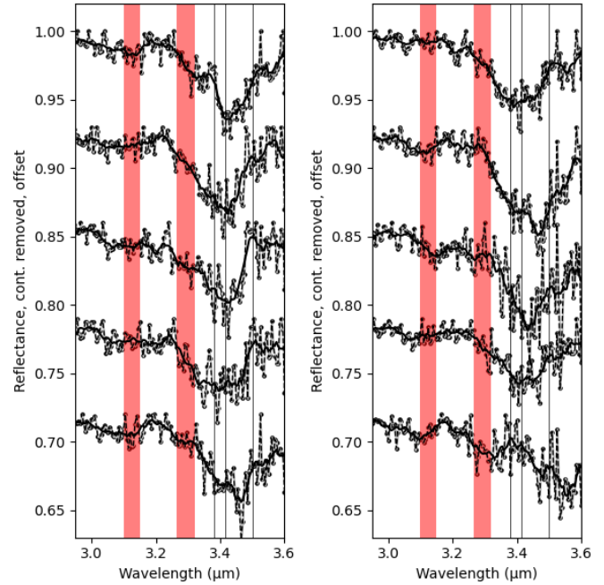
Fig. A.3. Example Bennu spectra that have a “shoulder” near 3.3\ \mu\text{m} that may be indicative of aromatic CH. Vertical lines at 3.10 , 3.275 , 3.38 , 3.42 , and 3.50\ \mu\text{m} indicate positions of possible absorption features.
