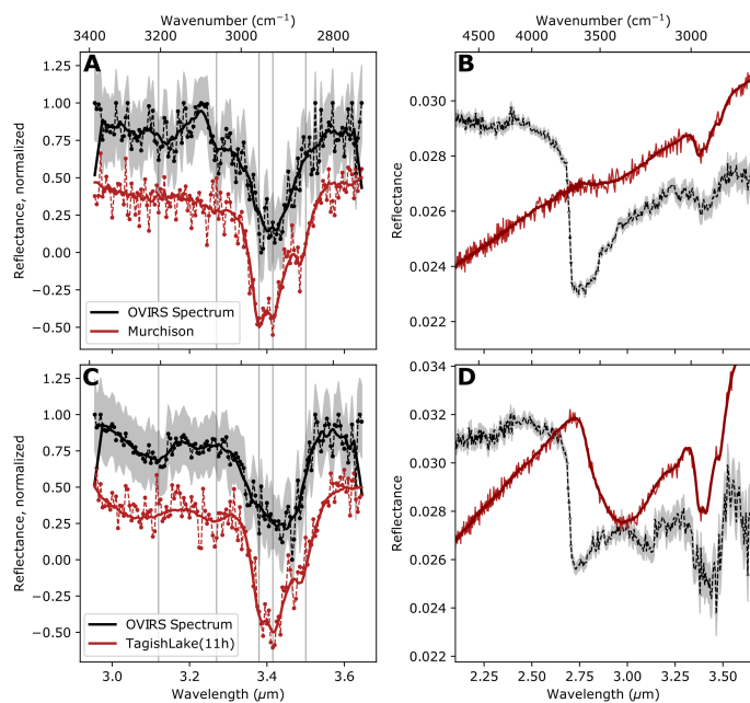
Fig. 2. Laboratory spectral matches for organic spectral shapes observed on Bennu. The most common spectral shapes in the Bennu spectra that we analyzed are well matched with spectra of meteorite IOM. (a) and (c) Best fits in the 3.1 to 3.6 \mu\text{m} region between the OVIRS spectra (black) and the IOM spectra (red, solid), with noised added to simulate OVIRS noise (red, dashed); the spectra are normalized from 0 to 1 and offset for clarity. The shaded region indicates uncertainties, and vertical lines at 3.10, 3.275, 3.38, 3.42, and 3.50 \mu\text{m} indicate positions of possible absorption features. (b) and (d) OVIRS and IOM spectra from 2.1 to 3.6 \mu\text{m} shown without normalization or continuum removal; IOM spectra have been scaled.
